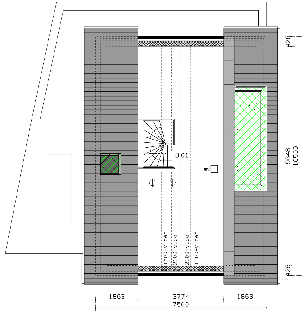
ZOLDER
